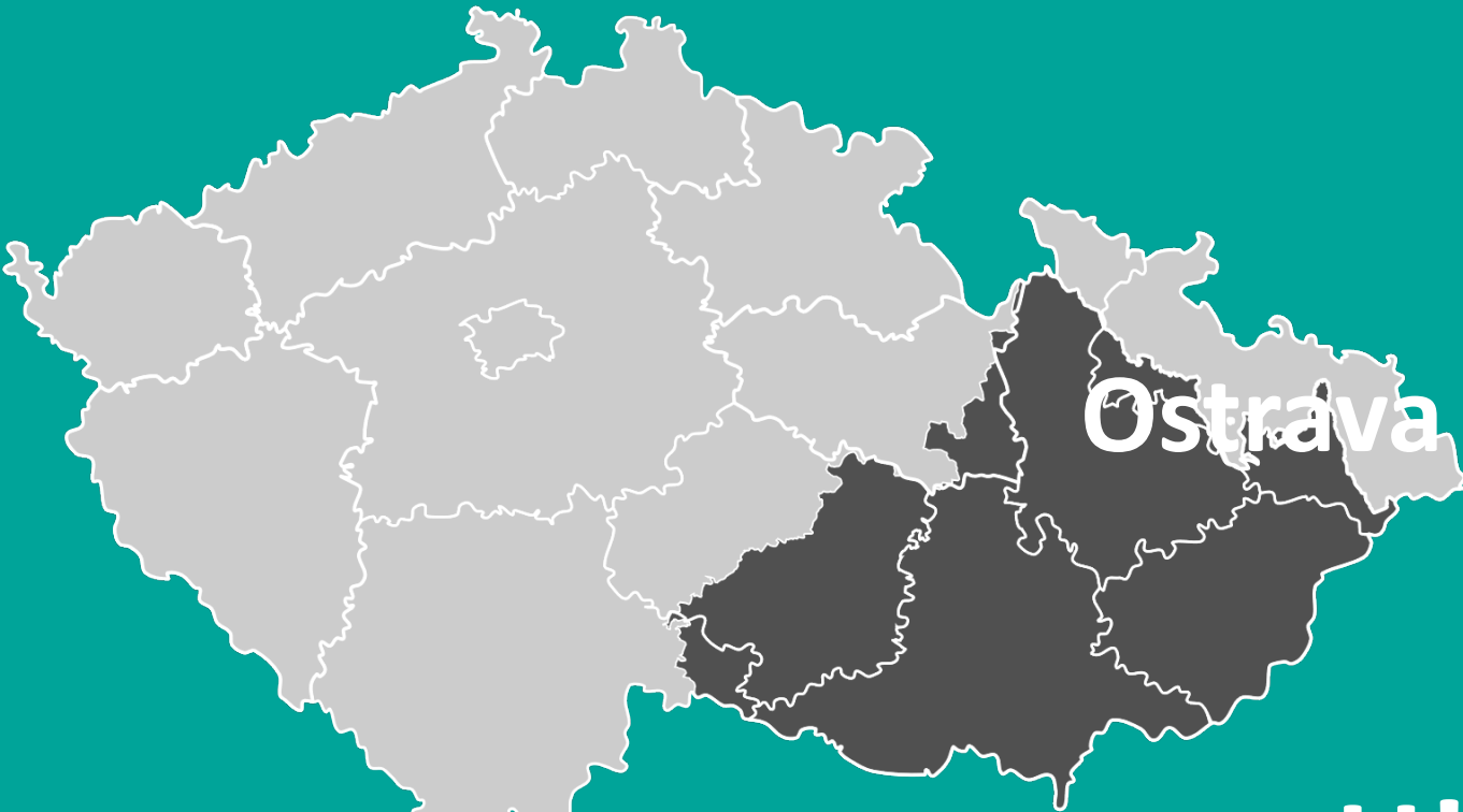
Location of Moravia within the Czech Republic, with modern admin region borders
